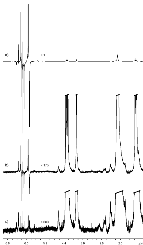
Figure 5. 200 MHz ^1\text{H} PASADENA NMR spectra recorded in situ from the catalytic hydrogenation of ethyl propiolate to form ethyl acrylate (a) during the reaction with 36% spin-polarized p\text{-H}_2 , (b) during the reaction with t\text{-H}_2 , and (c) after the reaction with t\text{-H}_2 and complete relaxation of the hyperpolarization. The vertical scales of (b) and (c) are enlarged versus (a) by the factors posted. NMR signals are assigned as follows: 4.2 ppm, acetylene proton of ethyl propiolate; 3.8 and 1.2 ppm, ester group of ethyl propiolate; 6.5–5.8 ppm, vinyl moiety of ethyl acrylate; 4.6 and 2.4 ppm, ester group of the product ethyl acrylate; 2.0 ppm residual protons of the solvent acetone- d_6 .
