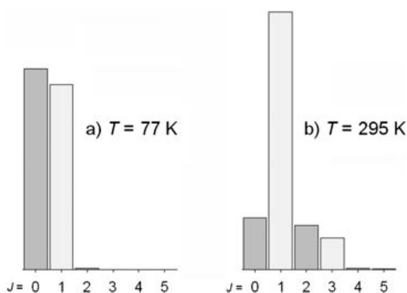
Figure 3. Partition histograms for the six lowest rotational states of \text{H}_2 at thermal equilibrium of (a) T = 77\text{ K} and (b) T = 295\text{ K} . Dark grey bars represent states of \text{p-H}_2 , while light grey bars refer to the states of \text{o-H}_2 . At 77\text{ K} , only the lowest two states (ground states for \text{p-H}_2 and \text{o-H}_2 ) and, at 295\text{ K} , only the lowest four rotational states are substantially populated. [16]
