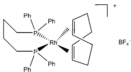
Scheme 1. [1,4-Bis(diphenylphosphino)butane](1,5-cyclooctadiene)rhodium(I) tetrafluoroborate.
