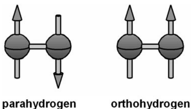
Figure 1. Very much simplified representation of the spin symmetry of p-H 2 and o-H 2 . The arrows in the H 2 ball-and-stick models symbolize effective magnetic moments. While this representation is probably a quantum mechanist's nightmare for it particularly violates Heisenberg's uncertainty relation, it still helps visualizing the antisymmetric (p-H 2 ) and symmetric (o-H 2 ) nuclear-spin wave function of H 2 .
