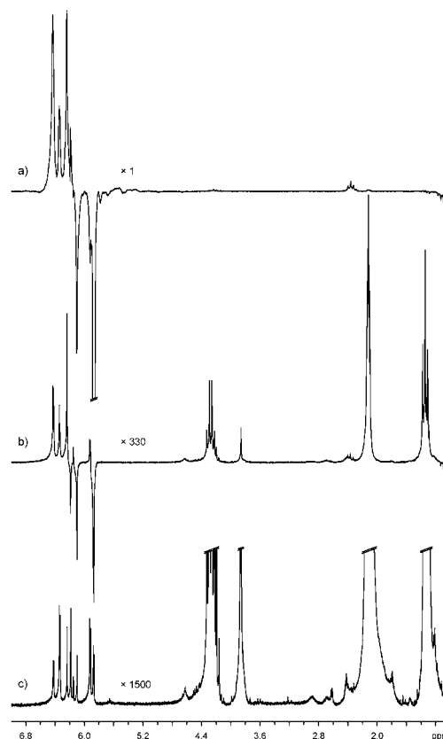
Figure 6. 200 MHz ^1\text{H} ALTADENA NMR spectra recorded from the catalytic hydrogenation of ethyl propiolate to form ethyl acrylate (a) during the reaction with 36% spin-polarized p\text{-H}_2 , (b) during the reaction with t\text{-H}_2 , and (c) after the reaction with t\text{-H}_2 and complete relaxation of the hyperpolarization. The vertical scales of (b) and (c) are enlarged versus (a) by the factors posted. NMR signals are assigned as explained in the legend to Figure 5. In addition, however, PHIP signals from the subsequent hydrogenation of ethyl acrylate to form ethyl propionate are observed in (a) and (b) at 2.4 ppm and 0.8 ppm for the methylene and methyl group of the propionate, respectively.
