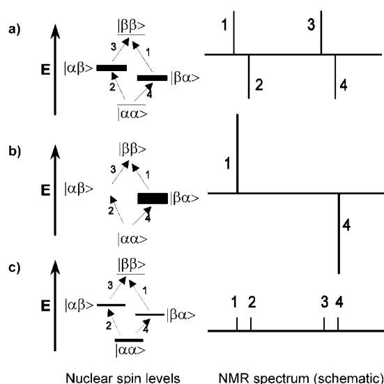
Figure 4. Spin-state diagram of hydrogen nuclei in an AX spin system (left). The populations are depicted by the line width of the states and yield the NMR spectra schematically shown on the right; (a) population and spectrum expected for PASADENA hydrogenation with pure p-H 2 , (b) population and spectrum expected for ALTADENA hydrogenation with pure p-H 2 , (c) population and spectrum expected after relaxation to thermal equilibrium.
