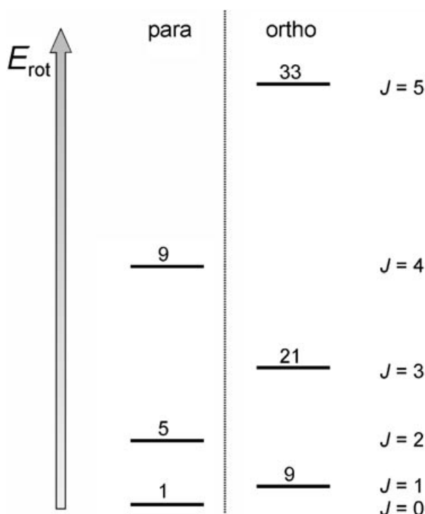
Figure 2. Lower rotational states of H 2 separated into columns of p-H 2 states (left) and o-H 2 states (right). The rotational quantum number ( J ) of each state is shown to the right of the columns, and the number of degeneracy is posted above each state.
